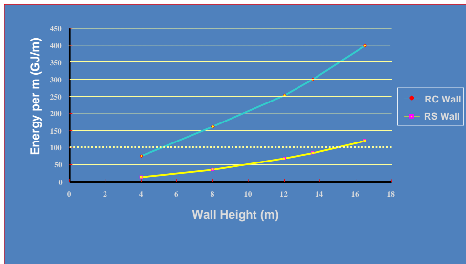
Figure 10. Comparison of the embodied energy of reinforced soil v reinforced concrete walls (After Geoguide 6, 2002)
